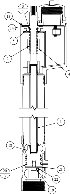
SECTION A-A CENTER SECTION VIEW
