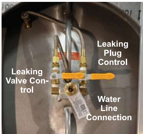
Manifold View
