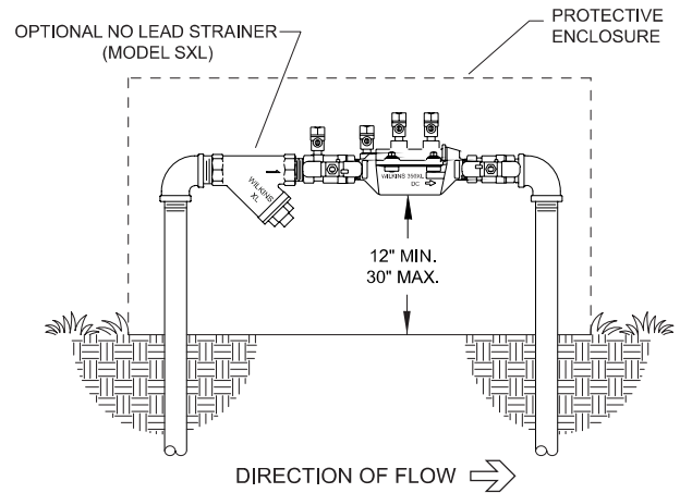
OUTDOOR INSTALLATION
