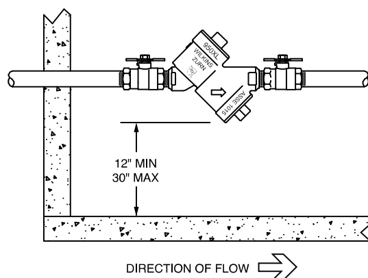
INDOOR INSTALLATION
