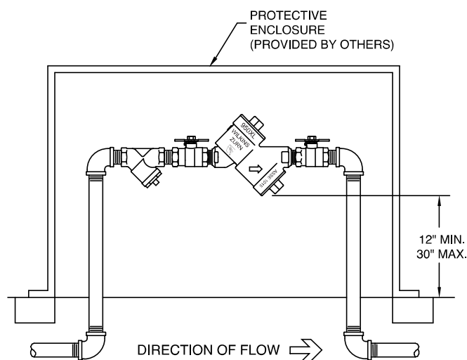
OUTDOOR INSTALLATION
