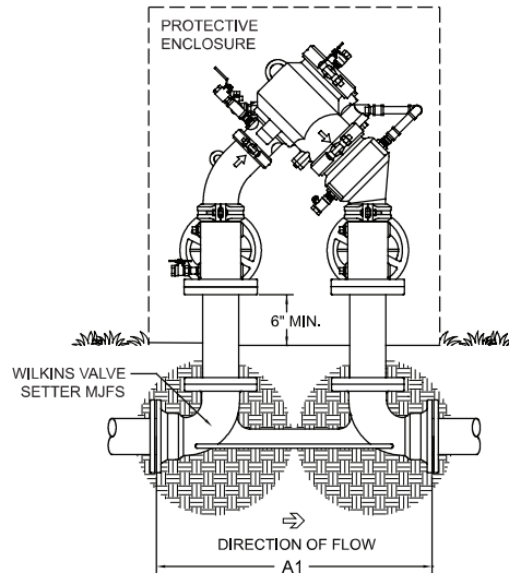
OUTDOOR INSTALLATION
