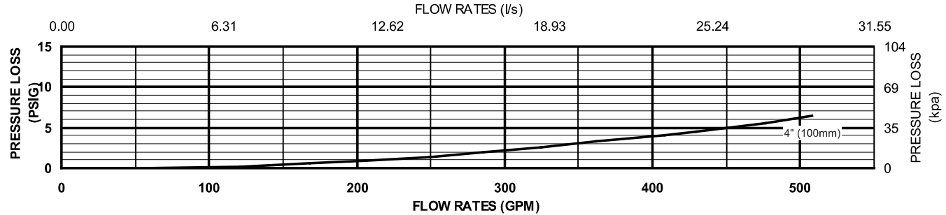
MODEL 40XL2 4"
