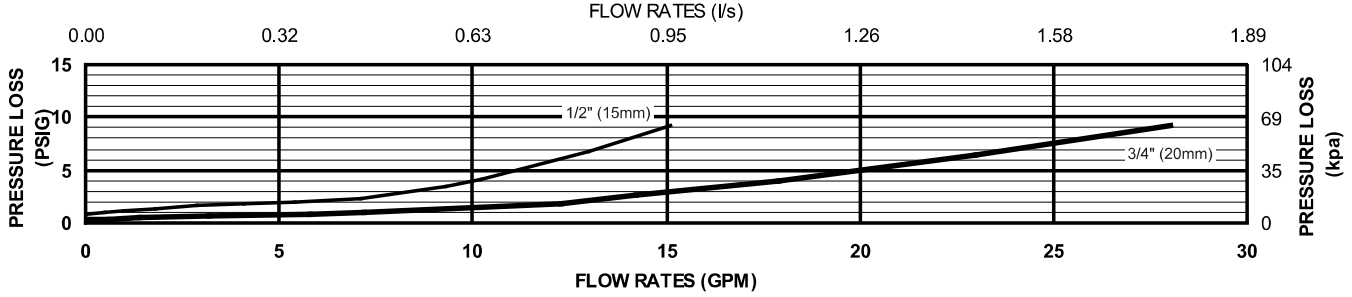
MODEL 40XL2 1/2" - 3/4"
