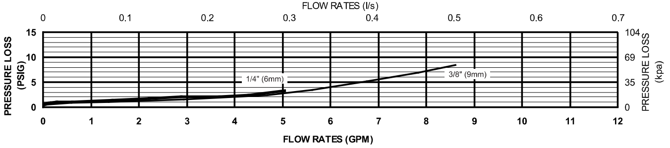
MODEL 40XL2 1/4" - 3/8"
