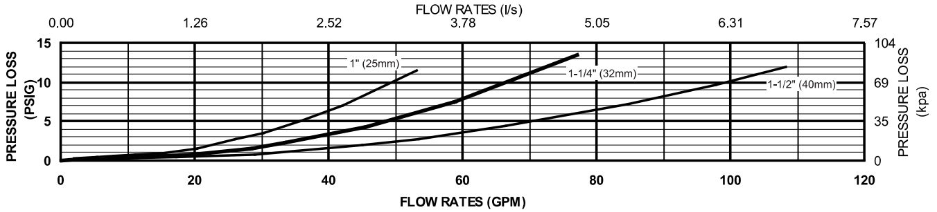
MODEL 40XL2 1" - 1 1/2"
