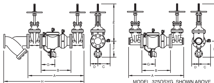
MODEL 375OSYG SHOWN ABOVE
