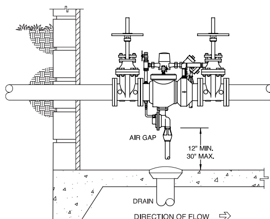
INDOOR INSTALLATION
