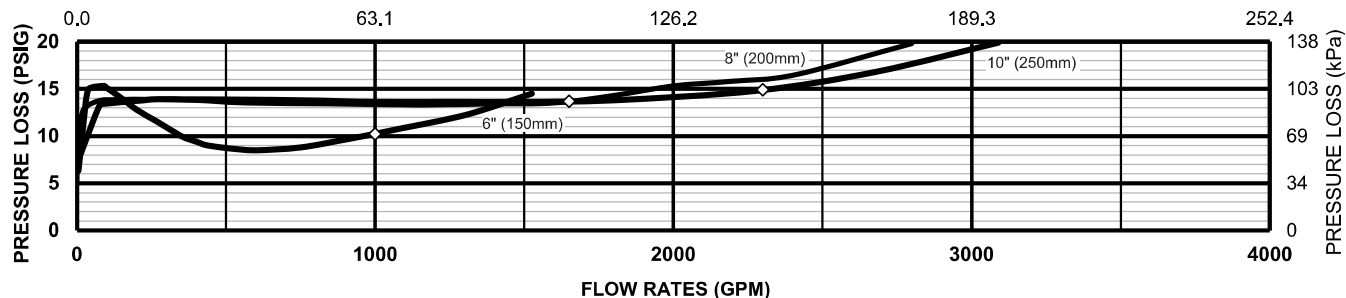
Capacity thru Schedule 40 Pipe (GPM)
