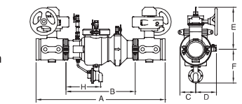
MODEL 375A with BG option
