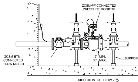
INDOOR INSTALLATION
