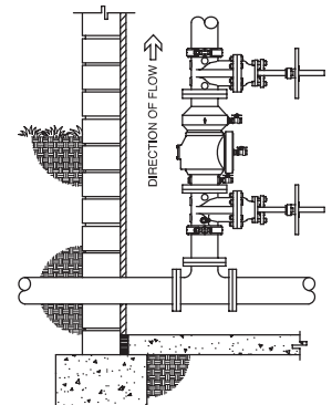
VERTICAL INSTALLATION (350OSY)
