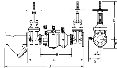
MODEL 350A with OSY & FSC option
