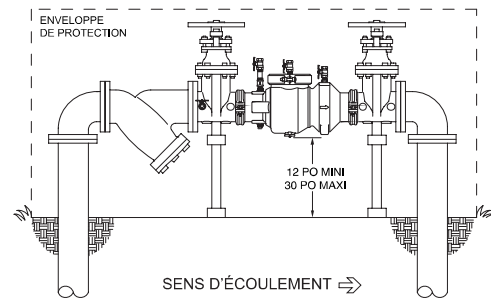
OUTDOOR INSTALLATION MODEL 350AFSC
