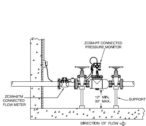
INDOOR INSTALLATION
