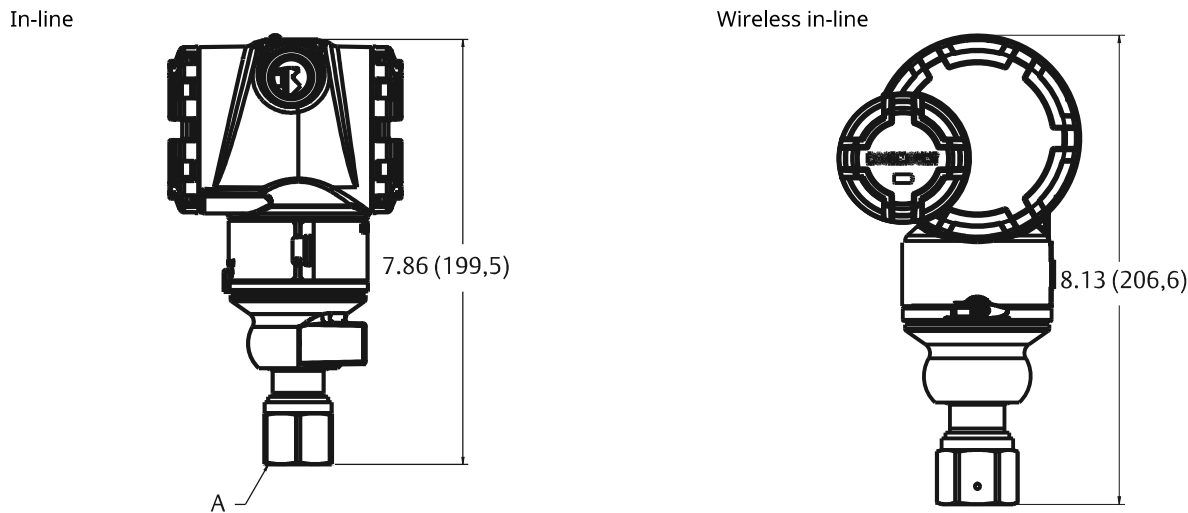
Figure 17: Rosemount 3051T In-Line Range 6
