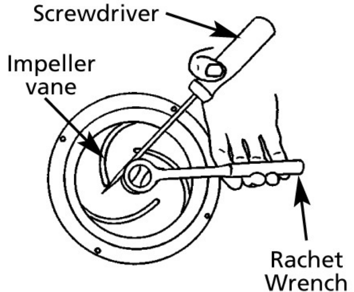
Figure 1 - Impeller Removal
