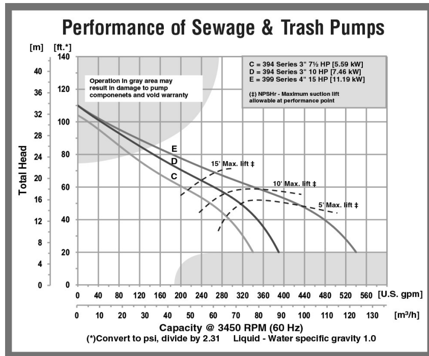
Figure 3 - Performance Curve
