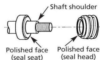
Figure 1 – Seal Replacement
