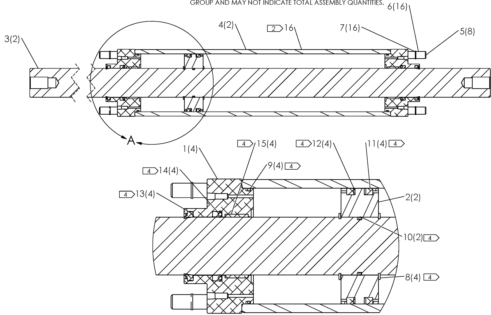
DETAIL A
